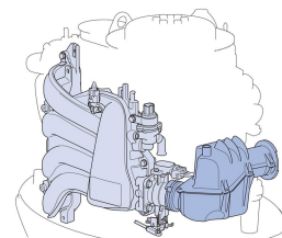
13_Throttle body, intake manifold and intake valves
